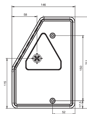
5 PIN BAYONET
